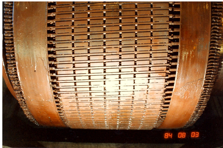
1350 KW D.C. Armature after rewind, reband and varnishing
